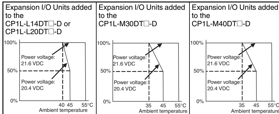
Relay Output Load Current Derating Curves for Expansion I/O Units
