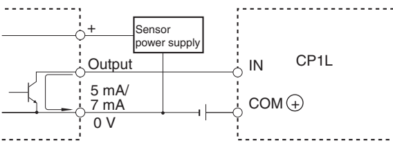
NPN open-collector output
