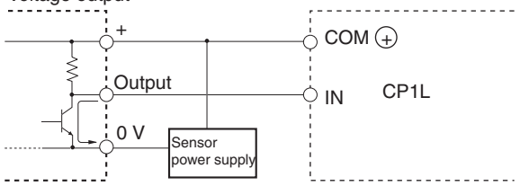
Voltage output
