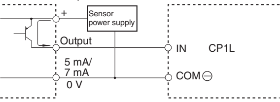
PNP current output
